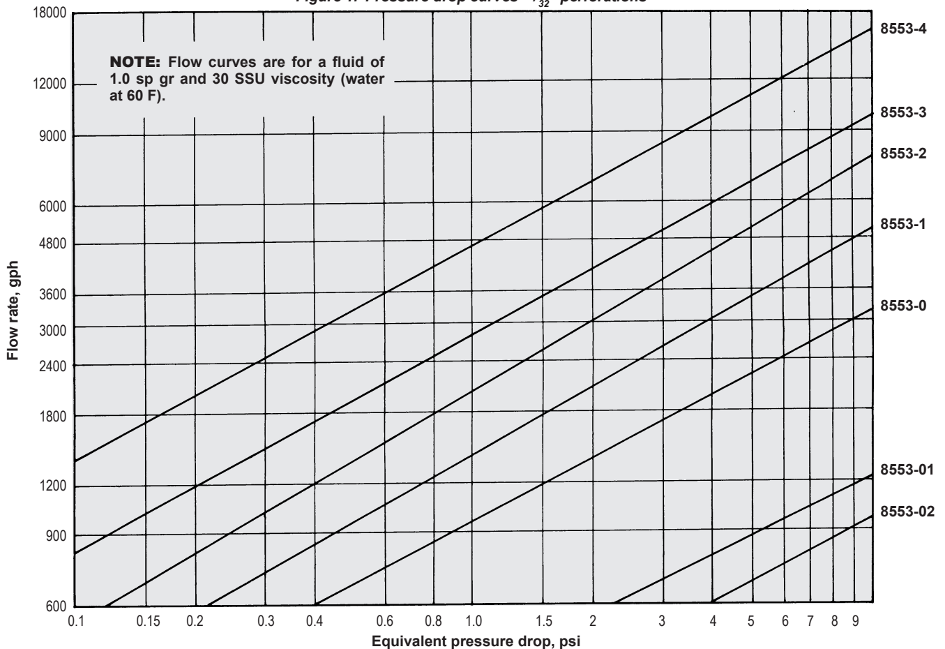
Figure 1. Pressure drop curves-- \frac{1}{32} " perforations
