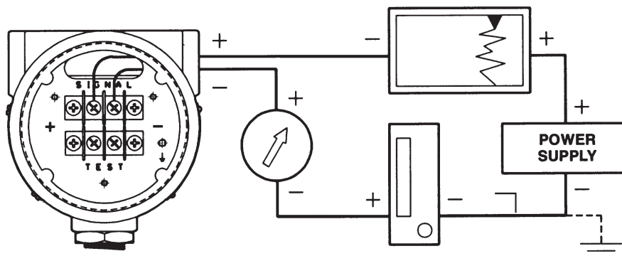
Signal loop must have 250 ohms minimum load for communications.
