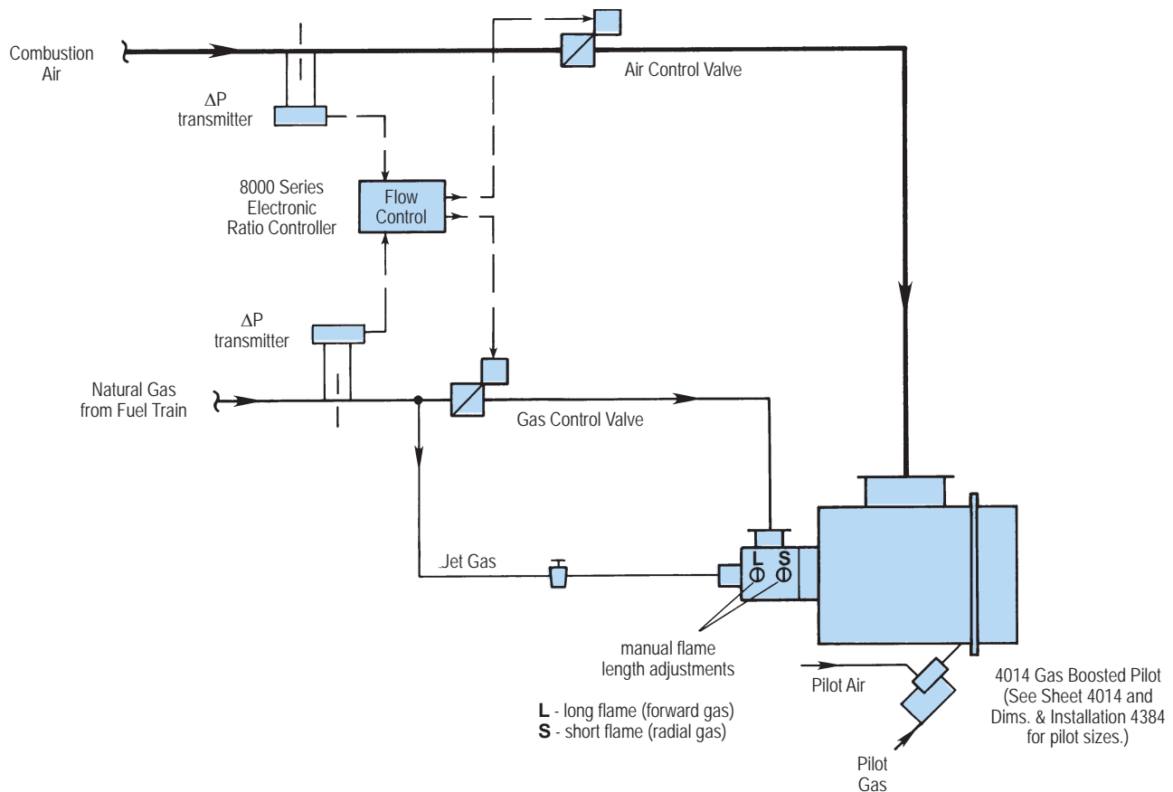
Typical Single Burner Fuel Directed Flow Control Schematic
