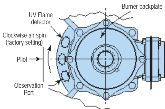
Figure 1. Proper ignition/flame detector placement
