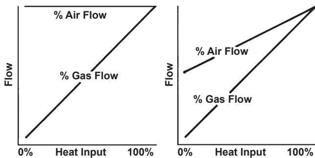
Figure 1. Constant air throttled fuel control.
