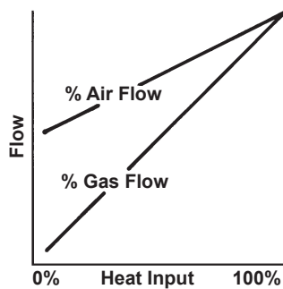
Figure 2. 7216 Regulator control.
