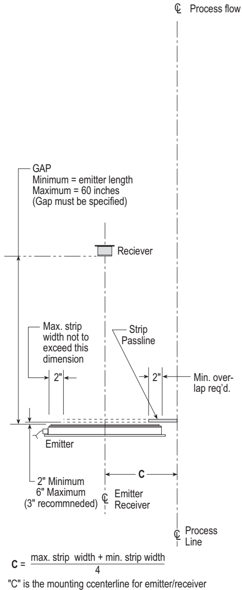
VIEW A-A FOR EDGE GUIDING
